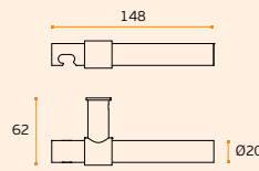
IN.00.146 FUNNY STOUT Material: EN 1.4301 - Satinado / Satin / Satin RB08M - Roseta standard / Standard rose Funny bottle opener
