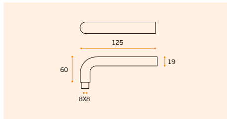
IN.00.028.P Material: EN 1.4301 - Polido / Polished / Pulido RB08M - Roseta standard / Standard rose
