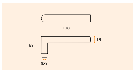
IN.00.030.P Material: EN 1.4301 - Polido / Polished / Pulido RB08M - Roseta standard / Standard rose
